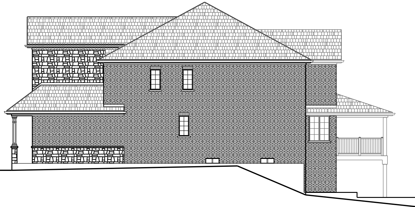
Right Side ( North ) Elevation
